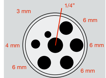
Multi-hole M02
