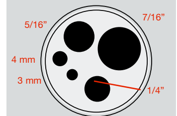
Multi-hole M10
