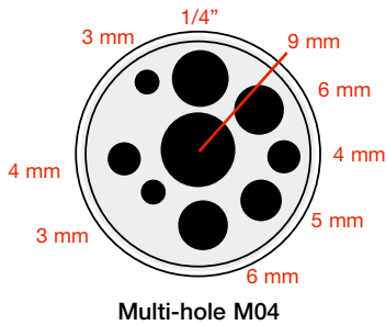
Multi-hole M04
