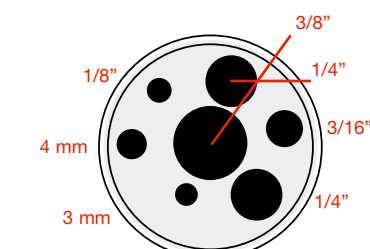
Multi-hole M06
